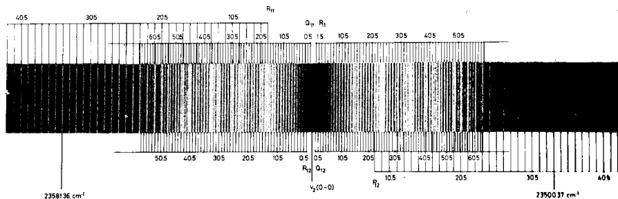
10.8 The fine structure of the 0-0 emission band of BeI, arising from the electronic transition A^2\Pi_{1/2} - X^2\Sigma^+ . (By courtesy of R. Colin.)
